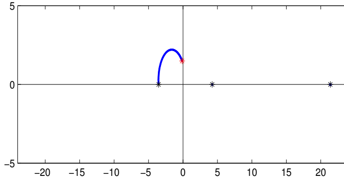
FIG. 7.4. Eigenvalue perturbation curves for the Hermitian pencil in Example 7.2 with respect to unstructured perturbation.
