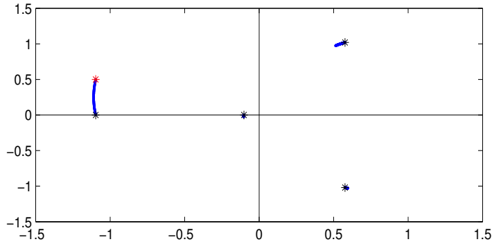
FIG. 7.2. Eigenvalue perturbation curves for the Hermitian pencil in Example 7.1 with respect to unstructured perturbation.
